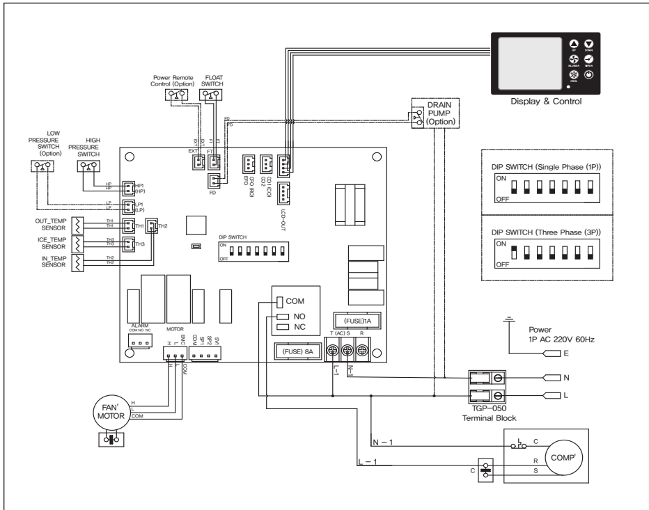
Figure 13 - Circuit Wiring Diagram (WPC-7000P)
